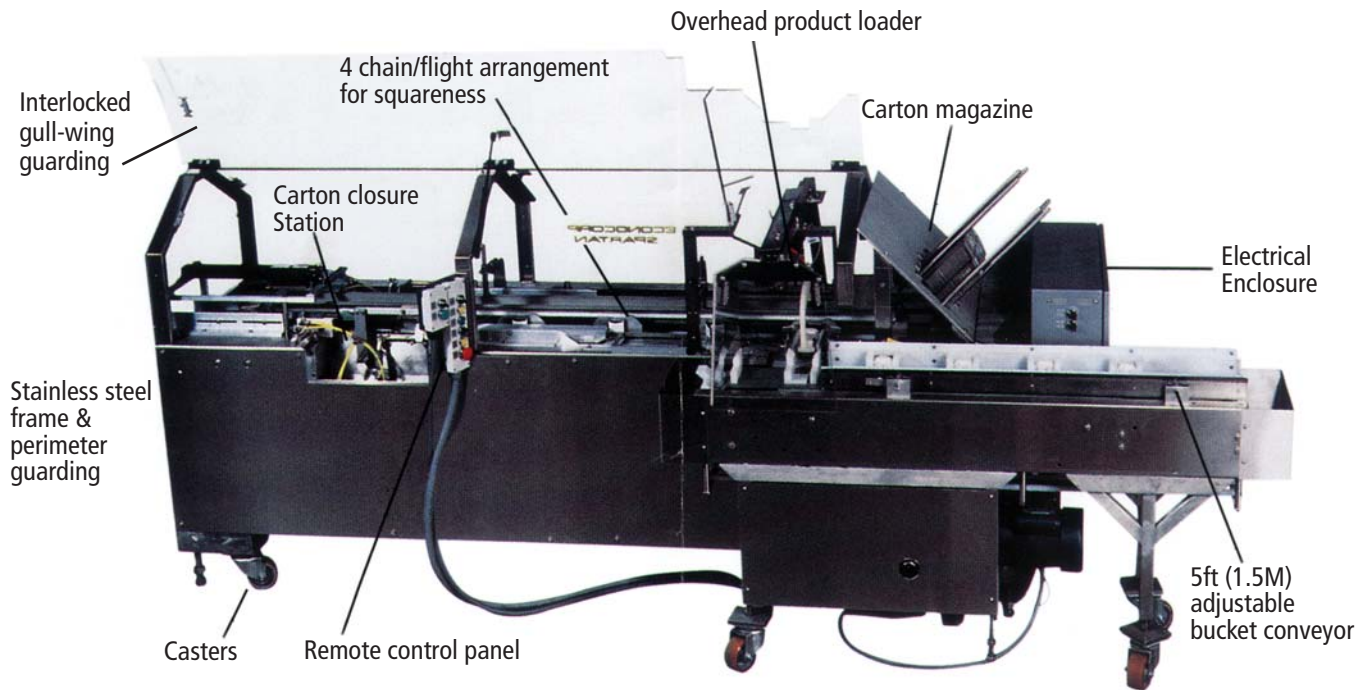
Spartan Cartoner shown with optional bucket conveyor and product loader.
